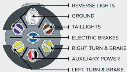
7 ROUND PIN
