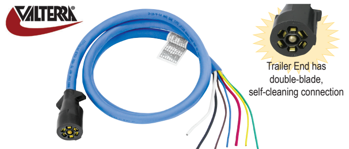
Trailer End has double-blade, self-cleaning connection
