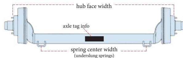
Drop Axle
