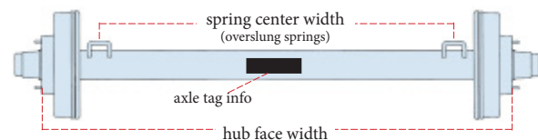
Straight Axle
